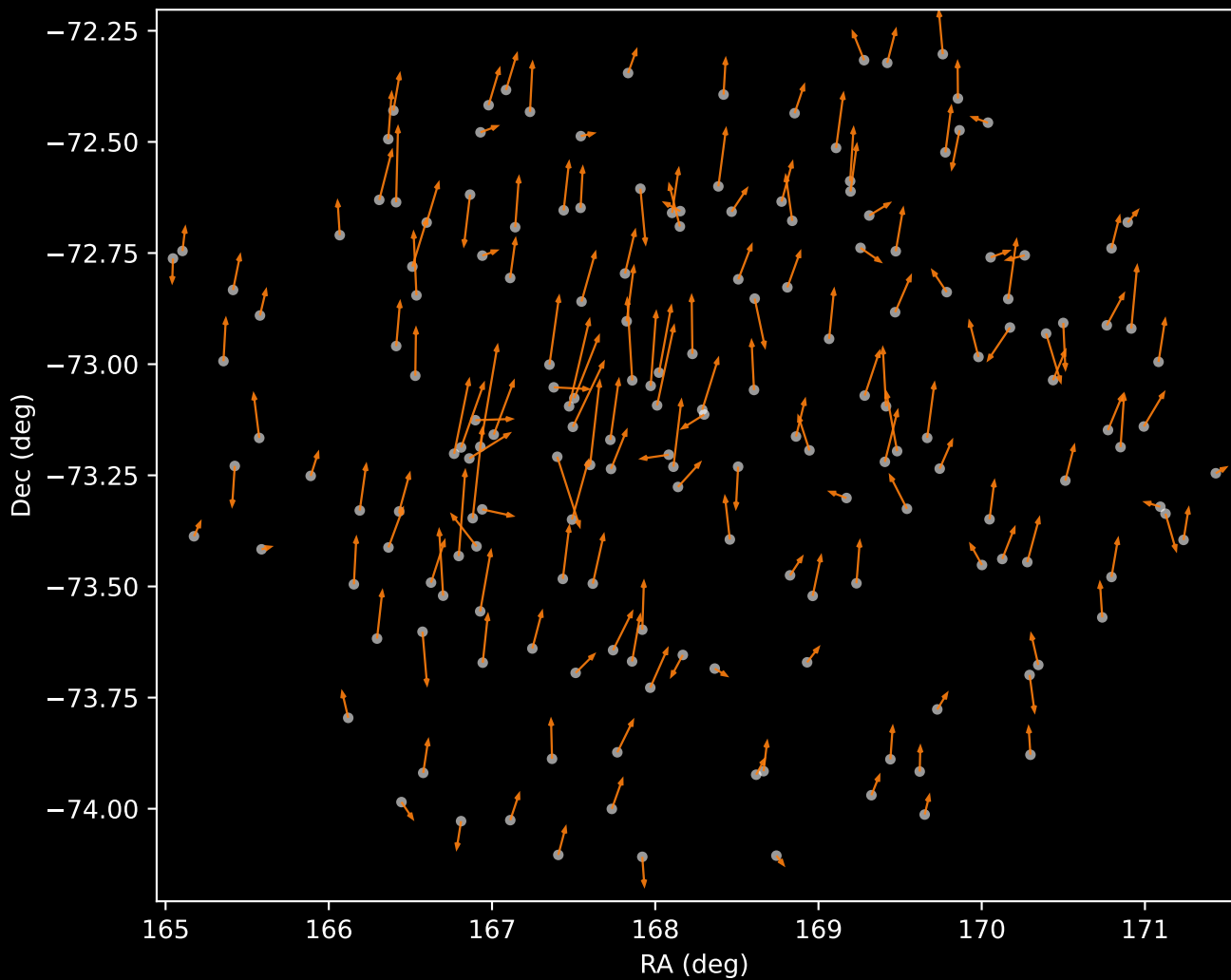
GALAH DR4 Cluster 2 Proper Motion Vectors (n=179)
