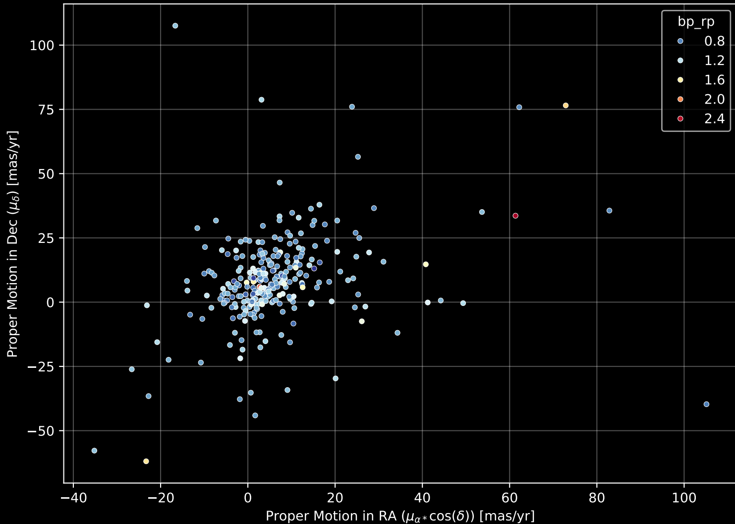
GALAH DR4 Field: [446] Proper Motion Diagram (n= 279)
