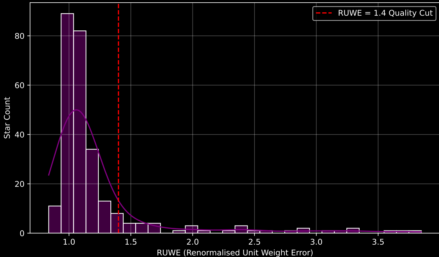
GALAH DR4 Field [446] RUWE Distribution (n= 270)
