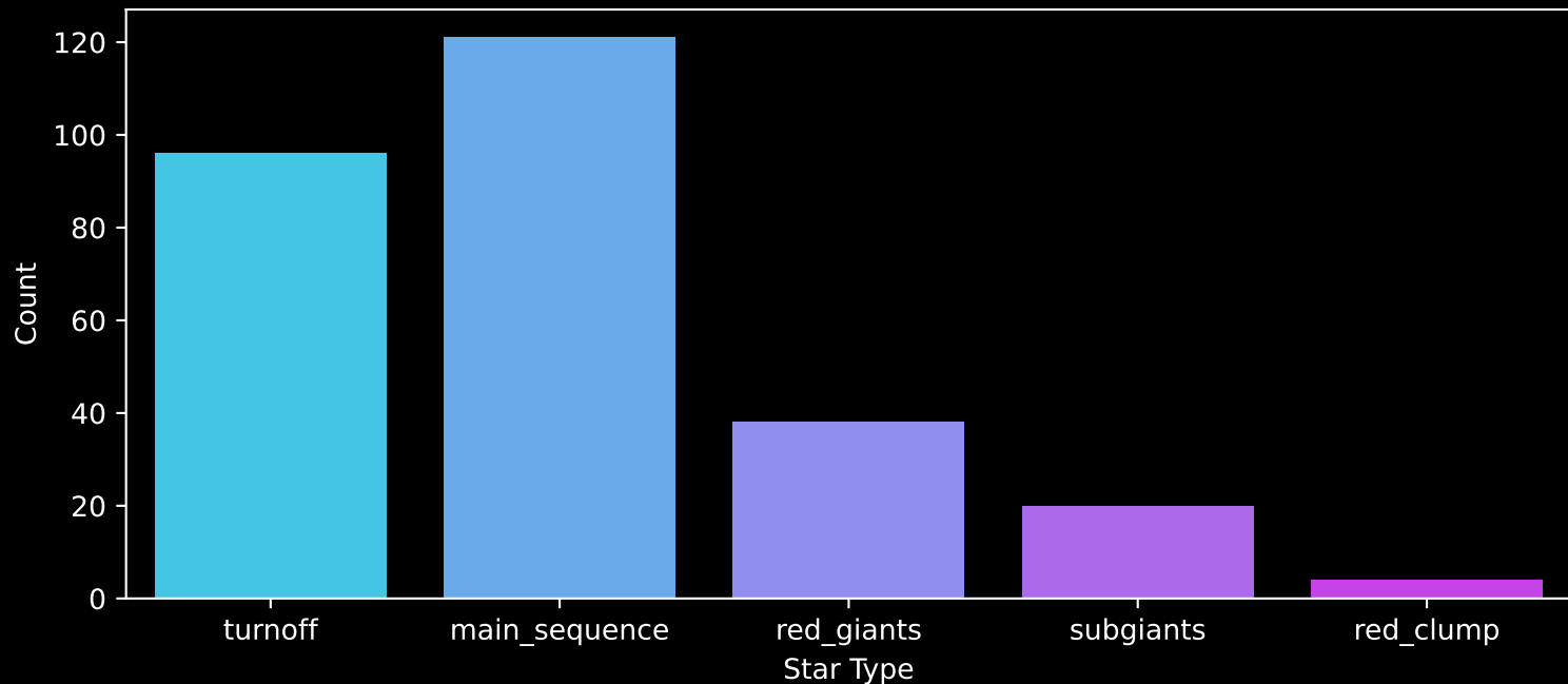
GALAH DR4 Field: [446] Count plot of Star Type
